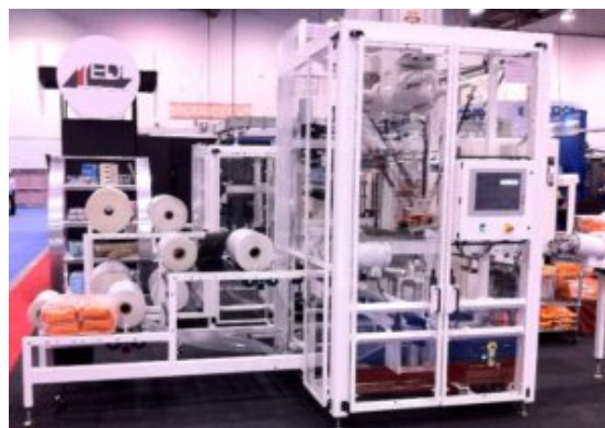
Double Tight Wrap with Vision Guided Robotics
