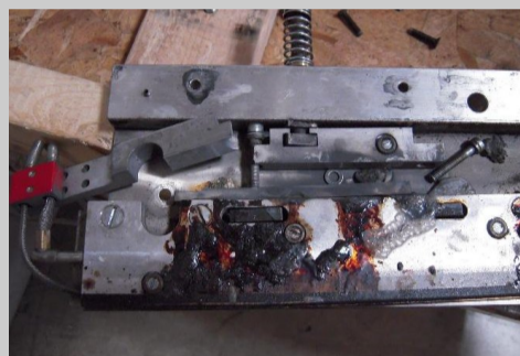
Seal Jaw - Before
